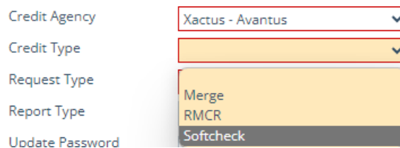
Figure 2: Softcheck (NEW)
